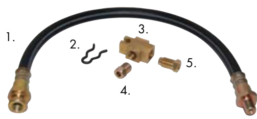
1. Flexible Brake Hose Part No. 920-840 2. Brake Hose Clip Part No. 920-850 3. Three Way Block Part No. 920-870 4. Tube Nut Short 3/8" Part No. 920-861
